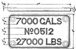
Figs. 4198-4199. Badge Plate.
